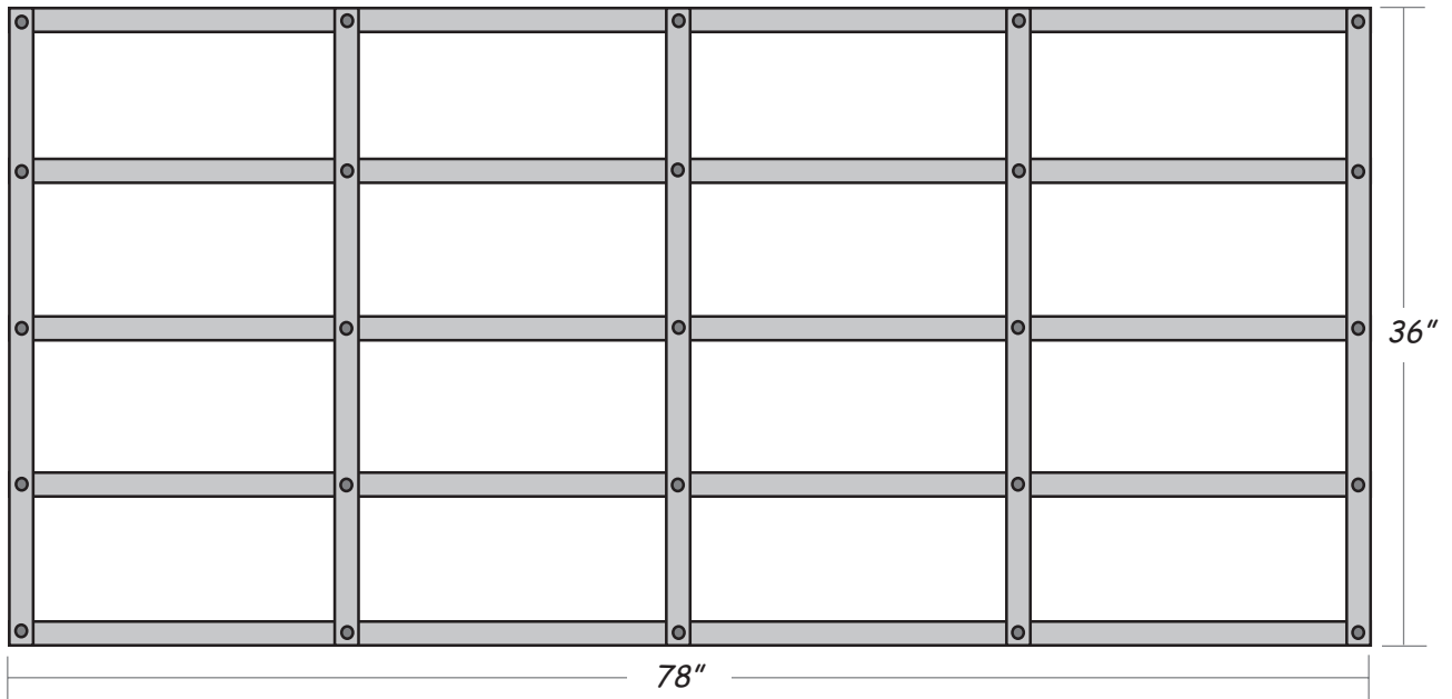
Fig. 1 - Build 4 pieces like this, from 1" X 2" lumber and 1 1/4" drywall screws
